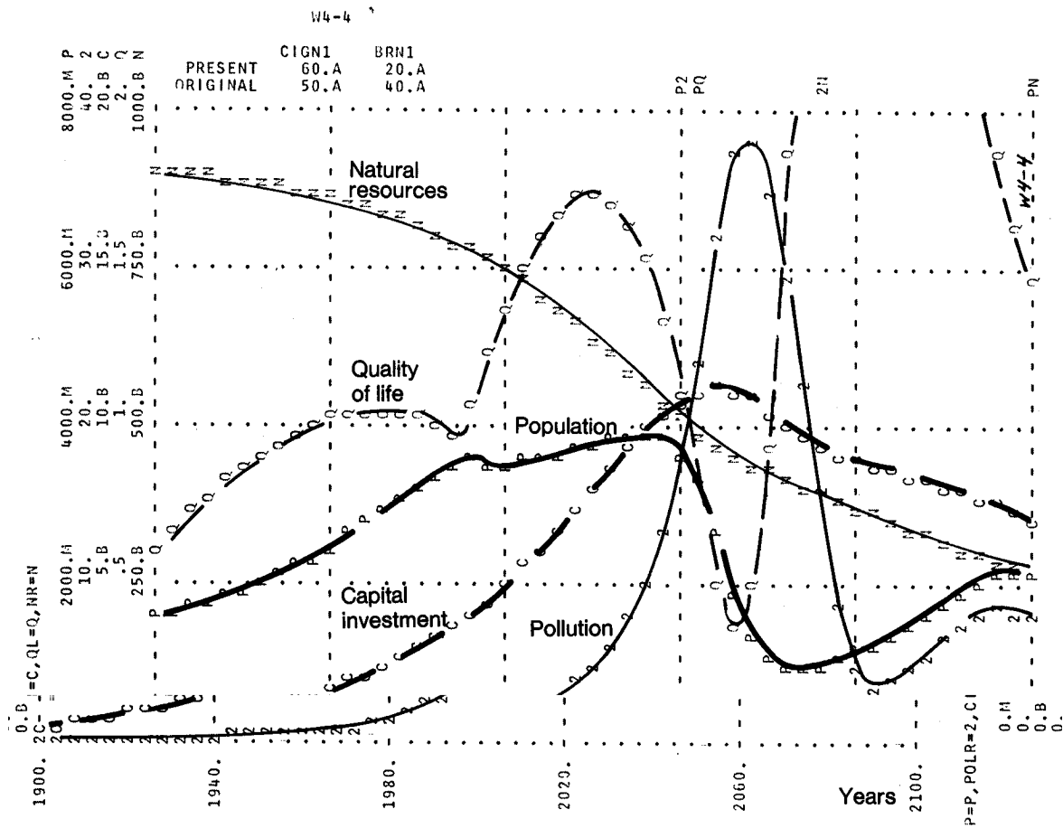
Fig. 5. In 1970 the 20 per cent increase in capital accumulation of Figure 4 is retained and “normal” birth rate is reduced 50 per cent. Capital investment continues to grow until a pollution crisis develops. After an initial decline, population is again pushed up by the rapid rise in quality of life that precedes the collapse.
